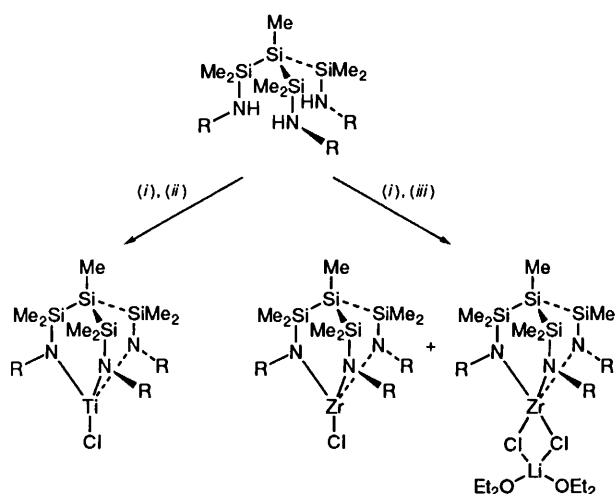
Scheme 1 Synthesis of the tripodal amido-titanium and -zirconium complexes. (i) 3 \text{LiBu}^n ; (ii) [\text{TiCl}_4(\text{thf})_2] ; (iii) \text{ZrCl}_4
